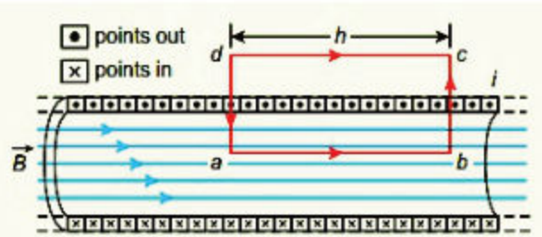
Figure 18.8 Amperian loop Solenoid
