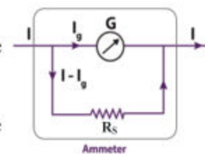
Figure 18.14 Ammeter and its schematic diagram
