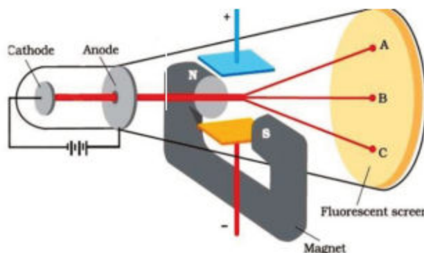
Figure 18.10 Cathode Ray Tube (CRT)
