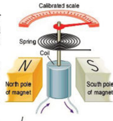
Figure 18.12 schematic diagram of Galvanometer
