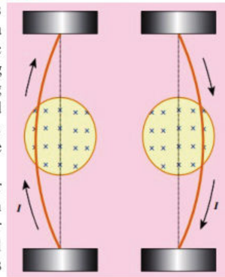
Figure 18.2 Magnetic Force on a current carrying conductor
