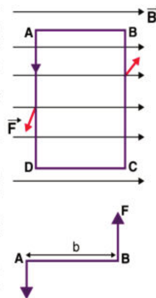
Figure 18.13 torque on rectangular coil
